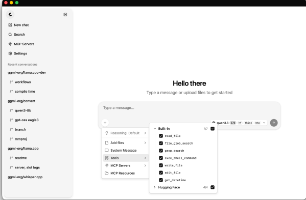
Built-in web UI against llama serve
